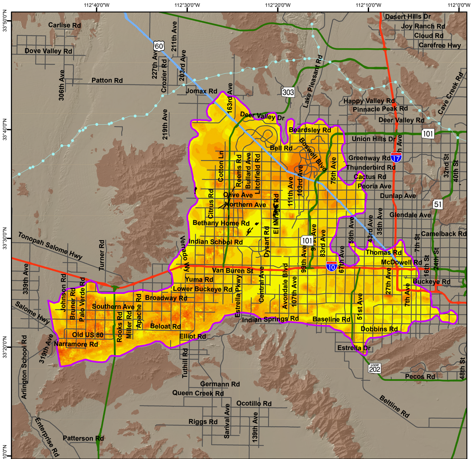
Total Land Subsidence in Western Metropolitan Phoenix, Maricopa County Based on Radarsat-2 Satellite Interferometric Synthetic Aperture Radar (InSAR) Data Time Period of Analysis: 16.0 Years 05/08/2010 To 04/02/2026
