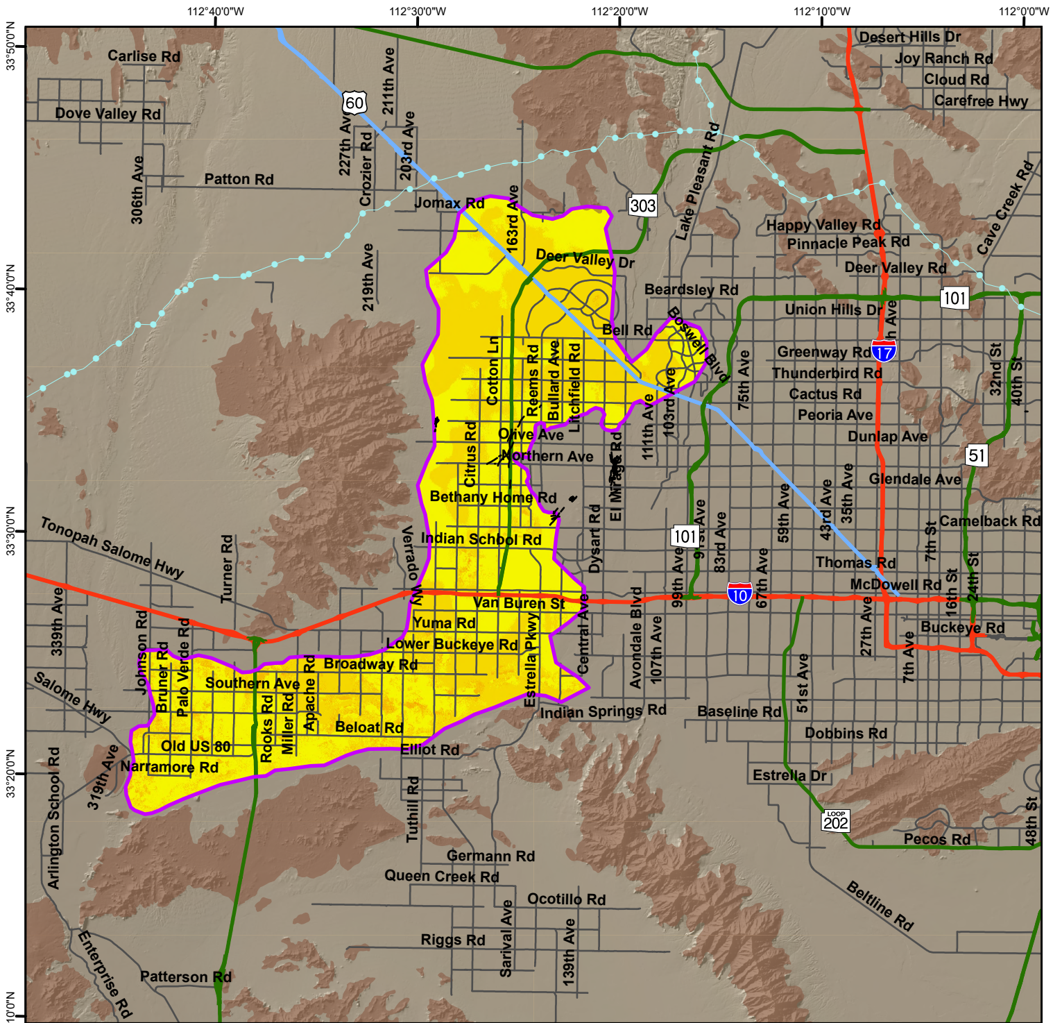
Total Land Subsidence in Western Metropolitan Phoenix, Maricopa County Based on Radarsat-2 Satellite Interferometric Synthetic Aperture Radar (InSAR) Data Time Period of Analysis: 2.0 Years 04/12/2024 To 04/02/2026
