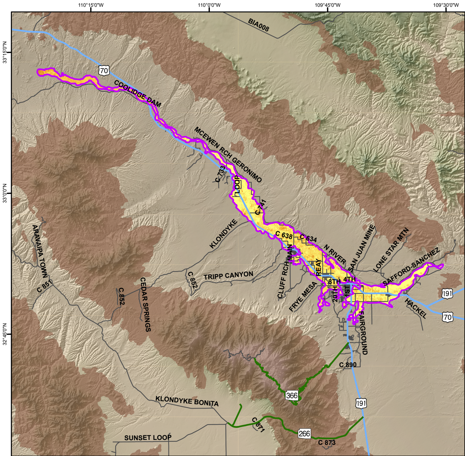
Land Subsidence Rate in the Upper Gila Area, Graham County Based on Sentinel-1 Satellite Interferometric Synthetic Aperture Radar (InSAR) Data Time Period of Analysis: 2.0 Years 05/08/2024 To 05/08/2026
