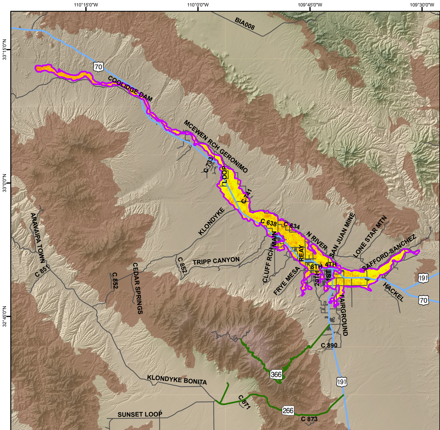
Total Land Subsidence in the Upper Gila Area, Graham County Based on Sentinel-1 Satellite Interferometric Synthetic Aperture Radar (InSAR) Data Time Period of Analysis: 2.0 Years 05/08/2024 To 05/08/2026
