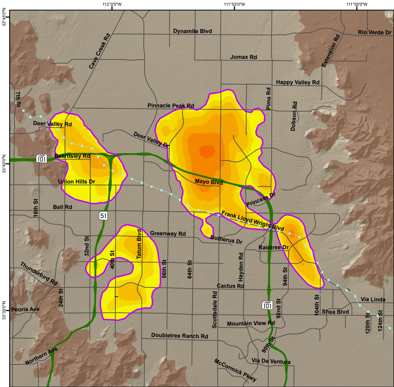
Total Land Subsidence in the Northeast Phoenix and Scottsdale Areas, Maricopa County Based on Radarsat-2 Satellite Interferometric Synthetic Aperture Radar (InSAR) Data Time Period of Analysis: 16.0 Years 05/08/2010 To 04/02/2026
