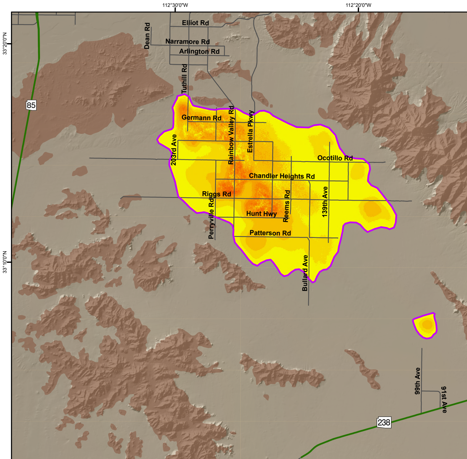
Total Land Subsidence in the Rainbow Valley Area, Maricopa County Based on Radarsat-2 Satellite Interferometric Synthetic Aperture Radar (InSAR) Data Time Period of Analysis: 16.0 Years 05/08/2010 To 04/02/2026
