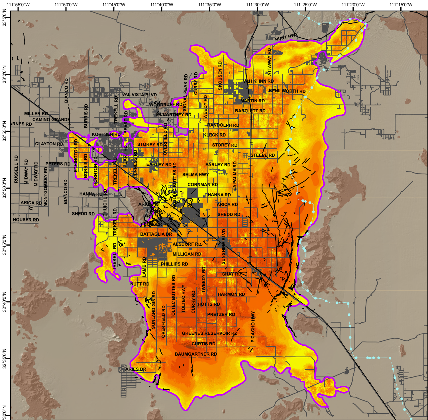
Total Land Subsidence in the Eloy Sub-Basin, Pinal County Based on Radarsat-2 Satellite Interferometric Synthetic Aperture Radar (InSAR) Data Time Period of Analysis: 16.0 Years 05/15/2010 To 03/16/2026
