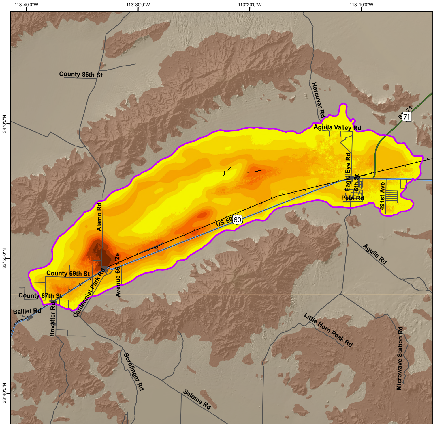
Total Land Subsidence in the McMullen Valley, La Paz and Maricopa Counties Based on Radarsat-2 Satellite Interferometric Synthetic Aperture Radar (InSAR) Data Time Period of Analysis: 16.0 Years 05/01/2010 to 03/26/2026
