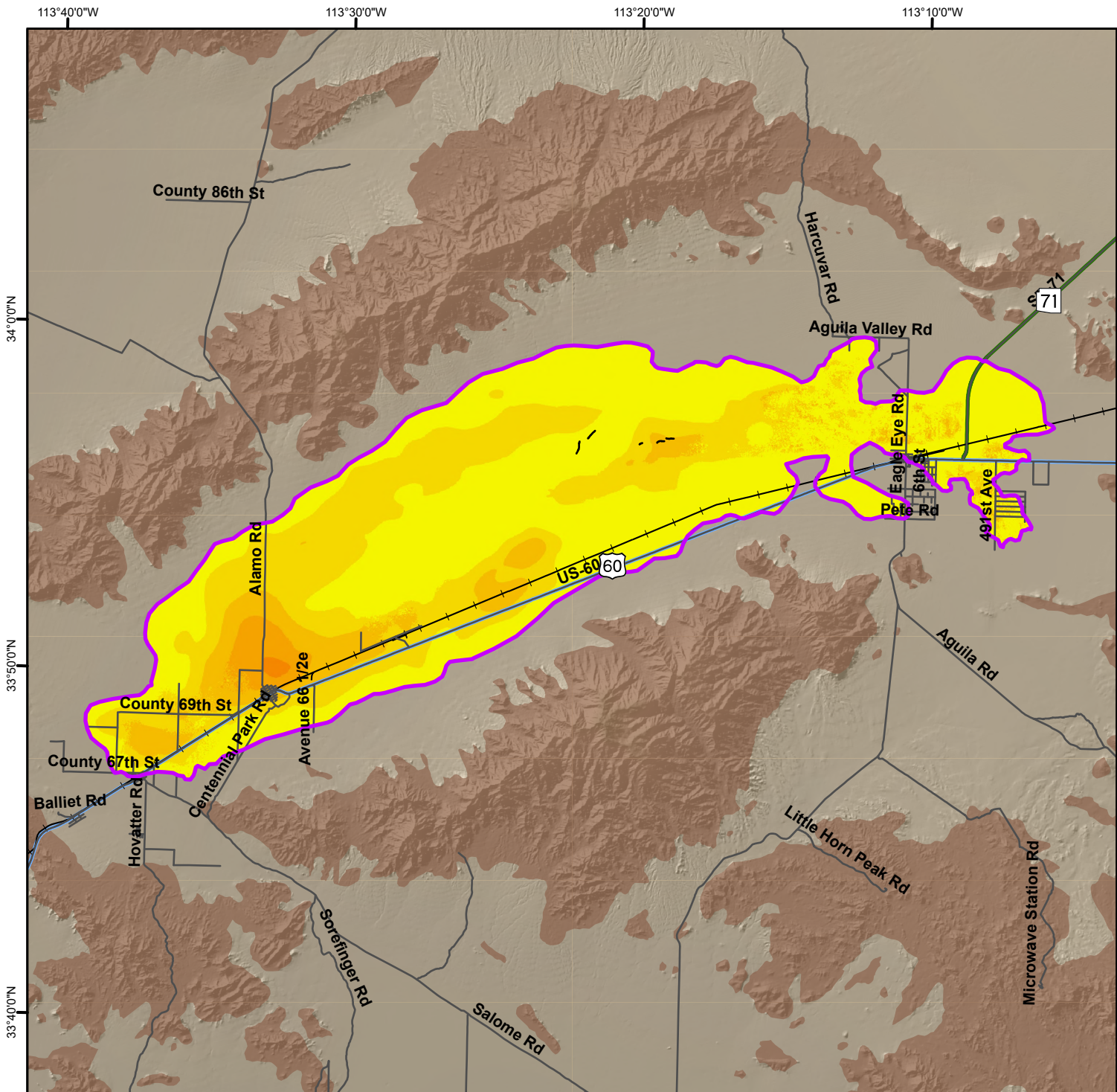
Total Land Subsidence in the McMullen Valley, La Paz and Maricopa Counties Based on Radarsat-2 Satellite Interferometric Synthetic Aperture Radar (InSAR) Data Time Period of Analysis: 1.0 Years 03/31/2025 to 03/26/2026
