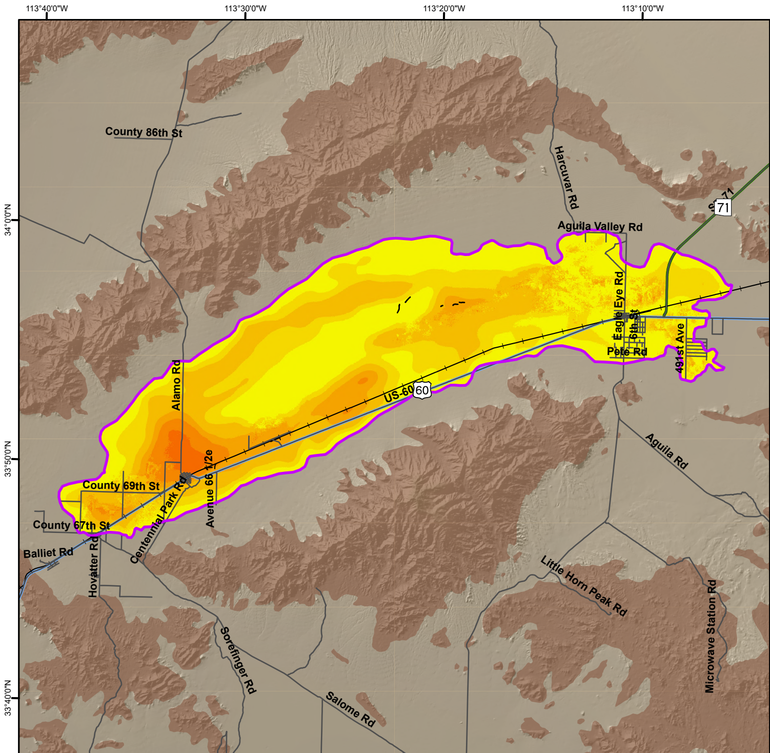
Total Land Subsidence in the McMullen Valley, La Paz and Maricopa Counties Based on Radarsat-2 Satellite Interferometric Synthetic Aperture Radar (InSAR) Data Time Period of Analysis: 2.0 Years 03/12/2024 to 03/26/2026
