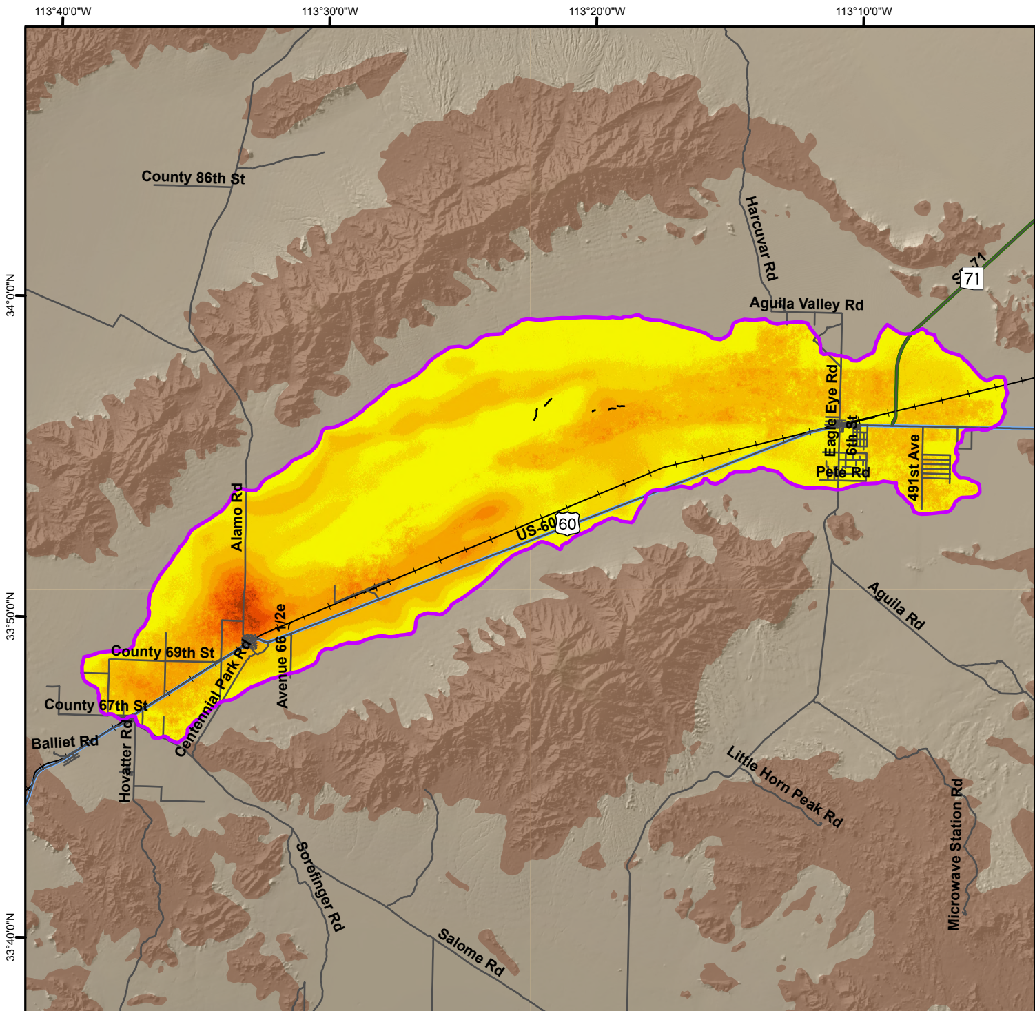
Total Land Subsidence in the McMullen Valley, La Paz and Maricopa Counties Based on Sentinel-1 Satellite Interferometric Synthetic Aperture Radar (InSAR) Data Time Period of Analysis: 9.0 Years 03/06/2017 To 04/24/2026
