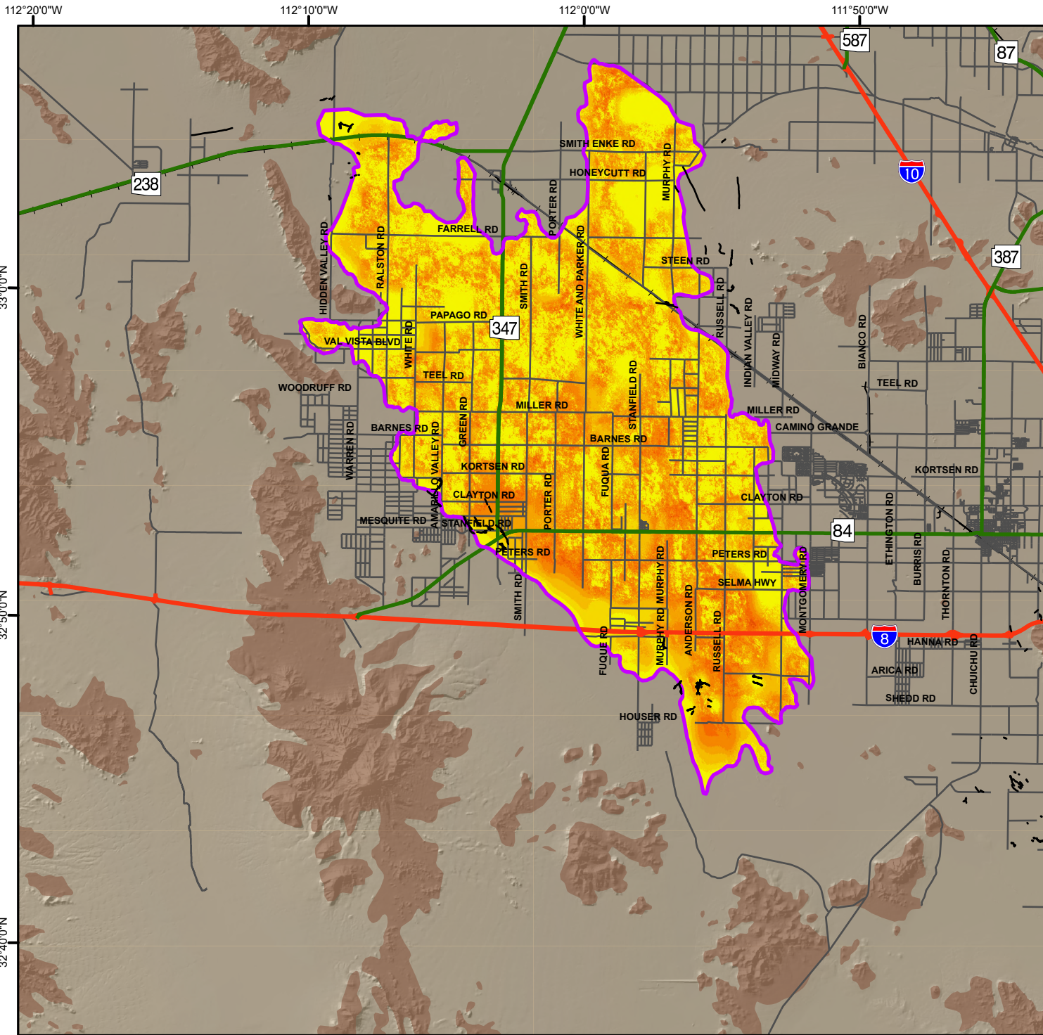
Total Land Subsidence in the Maricopa-Stanfield Sub-Basin, Pinal County Based on Radarsat-2 Satellite Interferometric Synthetic Aperture Radar (InSAR) Data Time Period of Analysis: 16.0 Years 05/08/2010 To 04/02/2026
