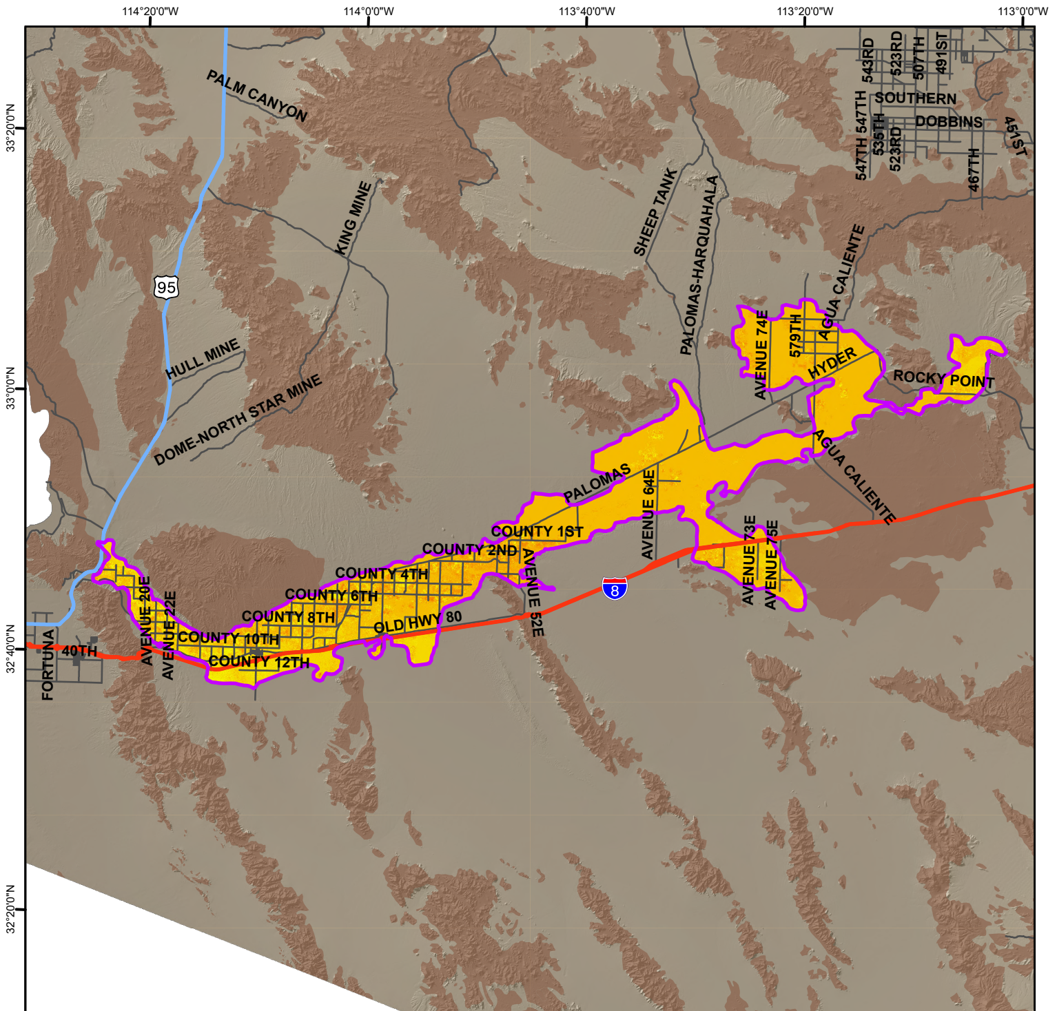
Total Land Subsidence in the Lower Gila Area, Maricopa and Yuma Counties Based on Sentinel-1 Satellite Interferometric Synthetic Aperture Radar (InSAR) Data Time Period of Analysis: 1.0 Years 05/23/2025 To 04/24/2026
