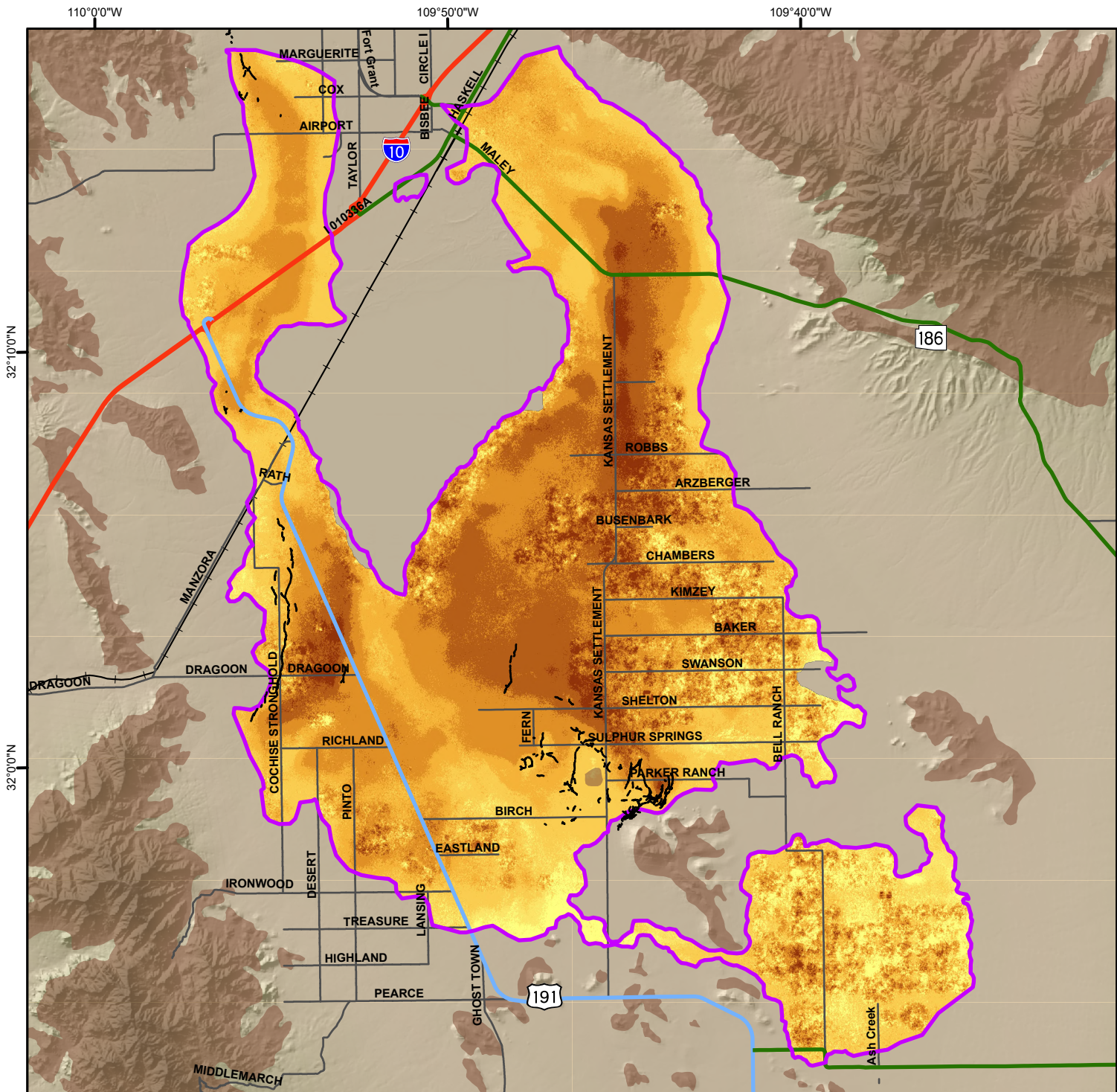
Land Subsidence Rate in the Willcox and Kansas Settlement Areas, Cochise County Based on Sentinel-1 Satellite Interferometric Synthetic Aperture Radar (InSAR) Data Time Period of Analysis: 1.0 Years 05/13/2025 To 05/08/2026
