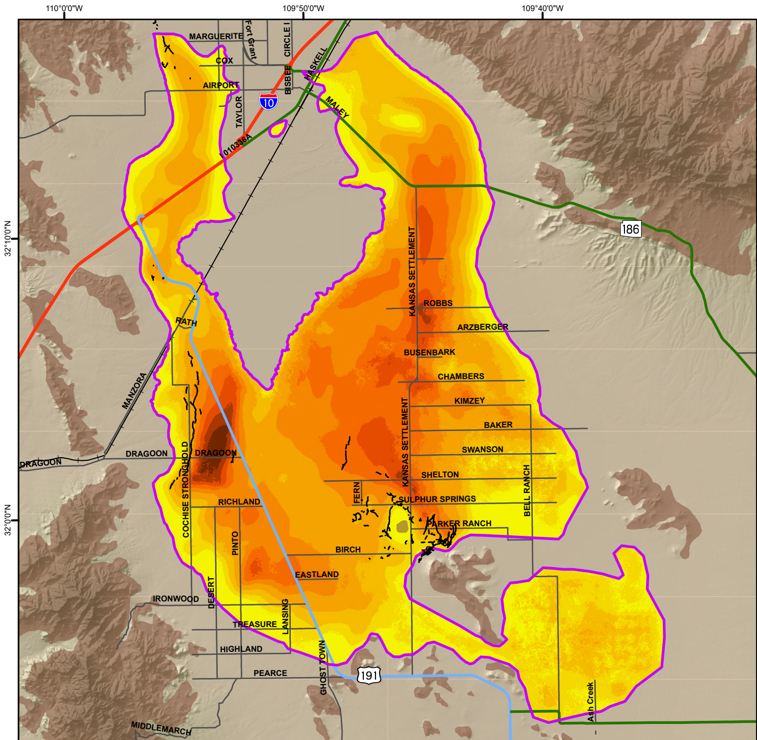
Total Land Subsidence in the Willcox and Kansas Settlement Areas, Cochise County Based on Radarsat-2 Satellite Interferometric Synthetic Aperture Radar (InSAR) Data Time Period of Analysis: 16.0 Years 05/05/2010 To 03/30/2026
