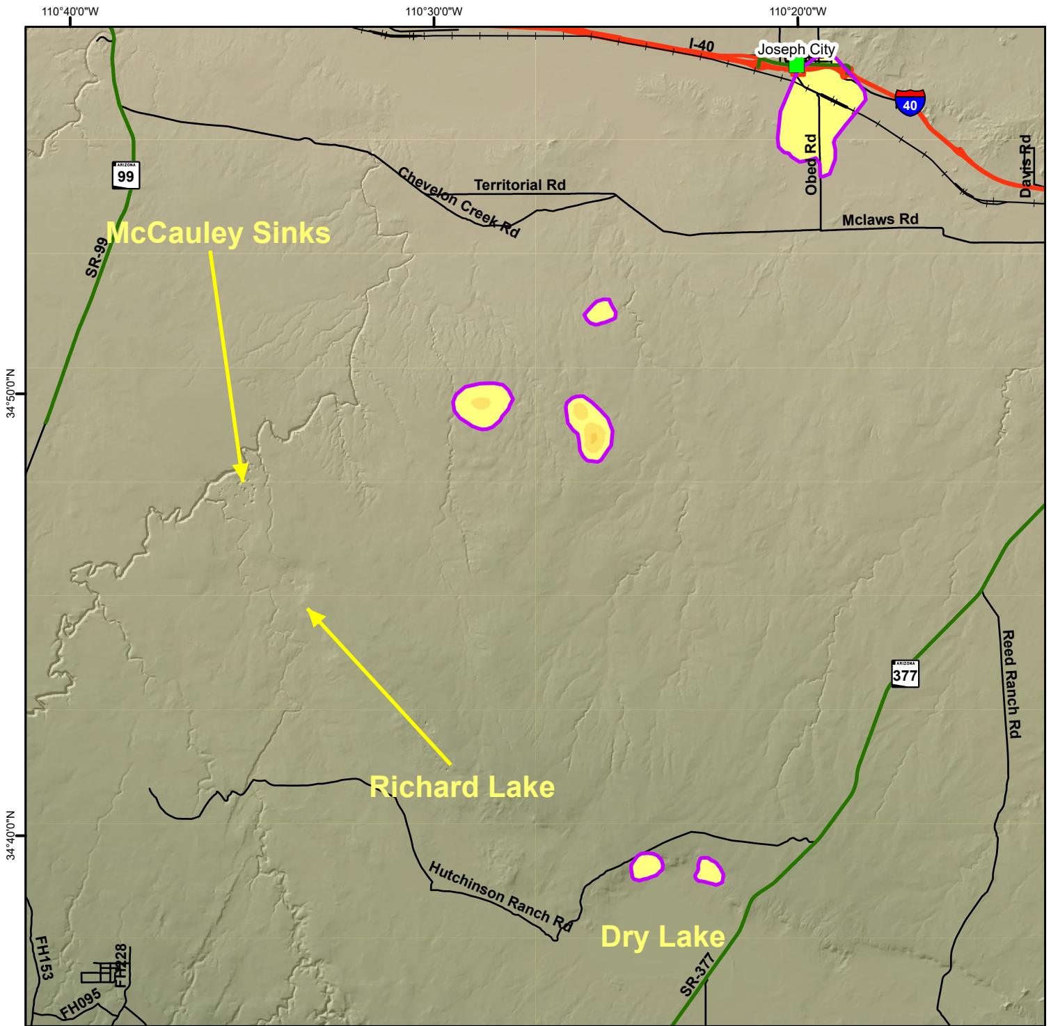
Land Subsidence Rate in the Holbrook Basin, Navajo County Based on Radarsat-2 Satellite Interferometric Synthetic Aperture Radar (InSAR) Data Time Period of Analysis: 1.9 Years 06/03/2024 To 04/03/2026
