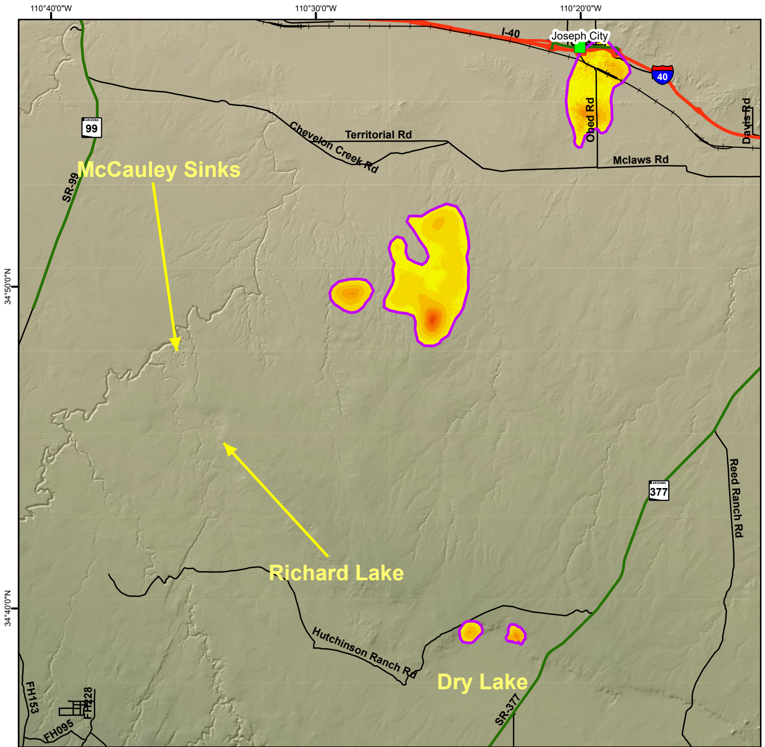
Total Land Subsidence in the Holbrook Basin, Navajo County Based on Radarsat-2 Satellite Interferometric Synthetic Aperture Radar (InSAR) Data Time Period of Analysis: 13.6 Years 09/22/2012 To 04/03/2026
