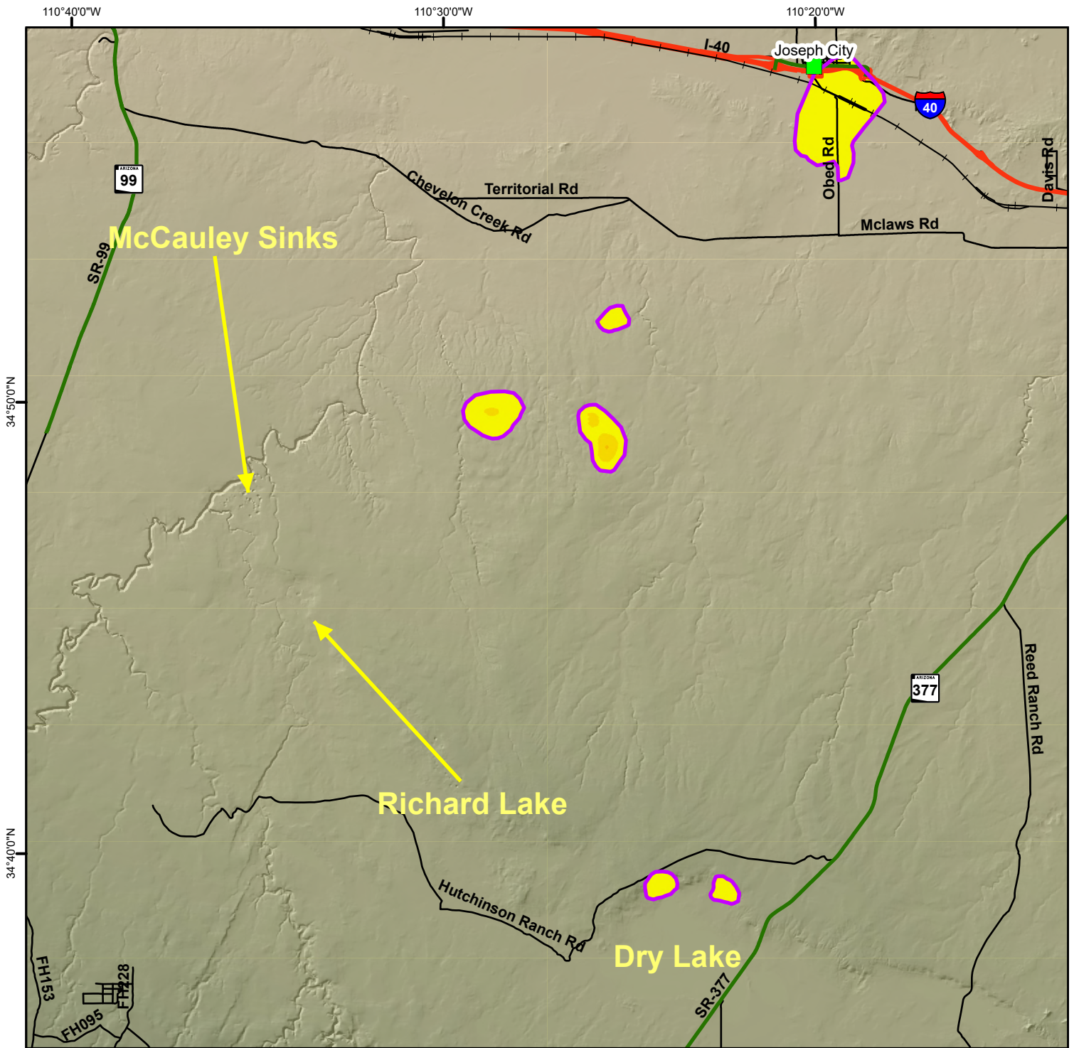
Total Land Subsidence in the Holbrook Basin, Navajo County Based on Radarsat-2 Satellite Interferometric Synthetic Aperture Radar (InSAR) Data Time Period of Analysis: 1.9 Years 06/03/2024 To 04/03/2026
