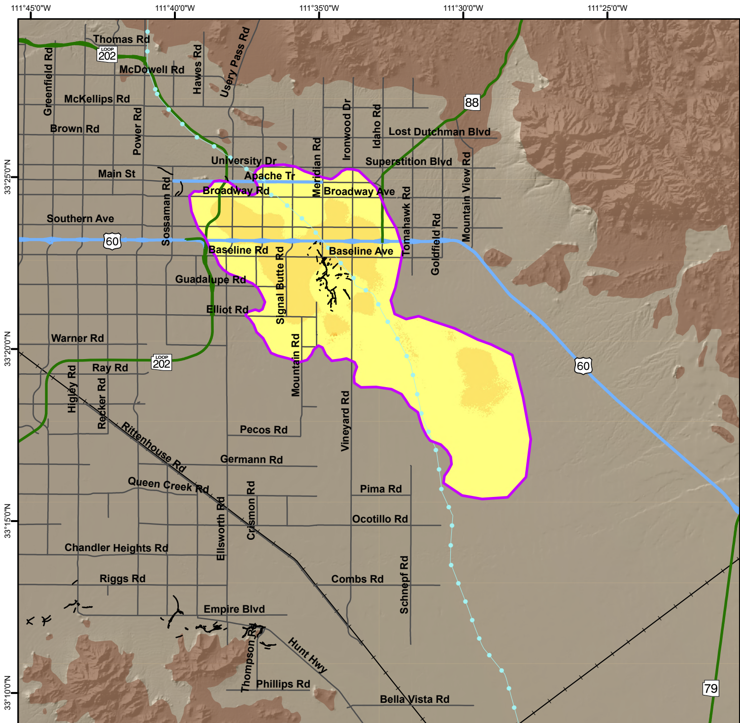
Land Subsidence Rate in the Hawk Rock Area, Maricopa and Pinal Counties Based on Radarsat-2 Satellite Interferometric Synthetic Aperture Radar (InSAR) Data Time Period of Analysis: 1.0 Years 03/21/2025 To 03/16/2026
