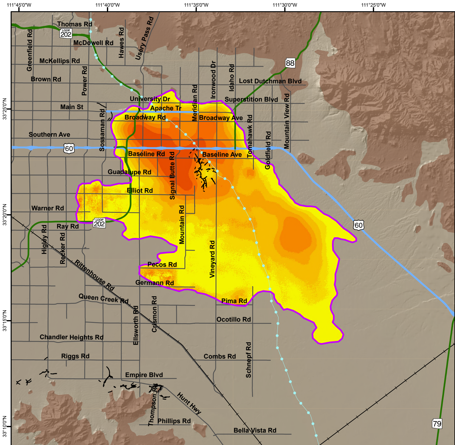
Total Land Subsidence in the Hawk Rock Area, Maricopa and Pinal Counties Based on Radarsat-2 Satellite Interferometric Synthetic Aperture Radar (InSAR) Data Time Period of Analysis: 16.0 Years 05/15/2010 To 03/16/2026
