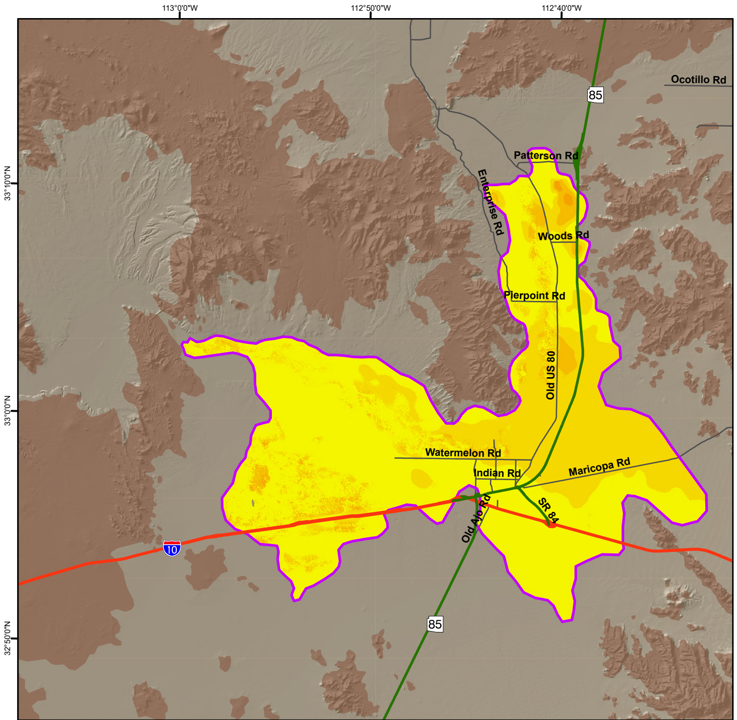
Total Land Subsidence in the Gila Bend Area, Maricopa County Based on Radarsat-2 Satellite Interferometric Synthetic Aperture Radar (InSAR) Data Time Period of Analysis: 2.0 Years 05/16/2024 To 05/06/2026
