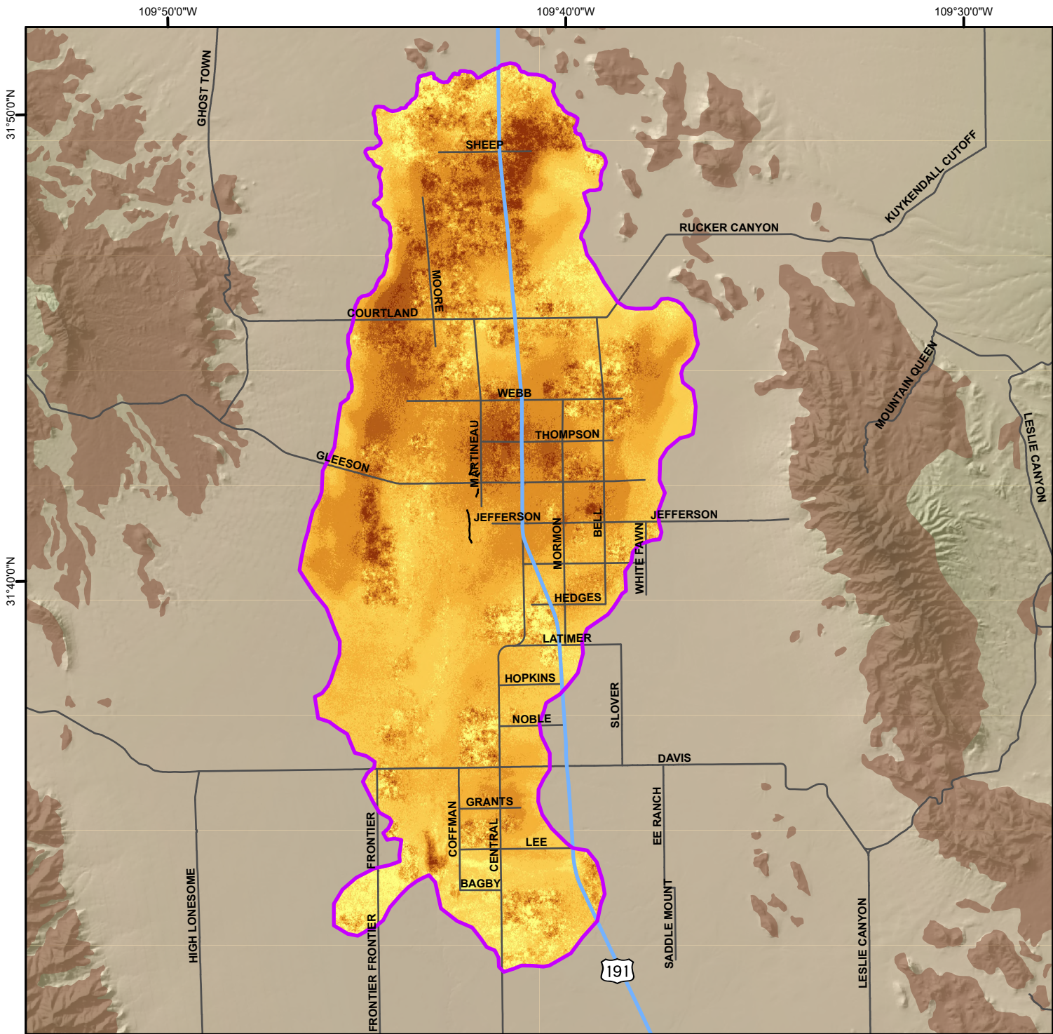
Land Subsidence Rate in the Elfrida Area, Cochise County Based on Sentinel-1 Satellite Interferometric Synthetic Aperture Radar (InSAR) Data Time Period of Analysis: 1.0 Years 05/13/2025 To 05/08/2026
