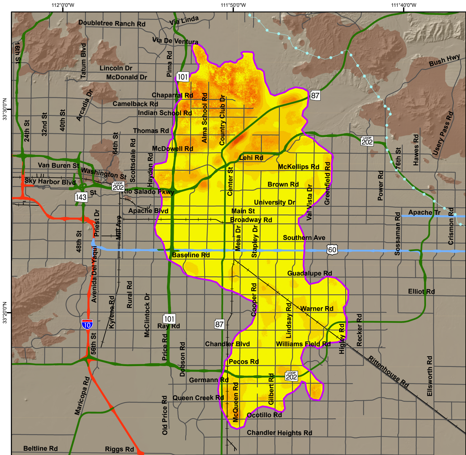
Total Land Subsidence in Eastern Metropolitan Phoenix, Maricopa County Based on Radarsat-2 Satellite Interferometric Synthetic Aperture Radar (InSAR) Data Time Period of Analysis: 16.0 Years 05/08/2010 To 04/02/2026
