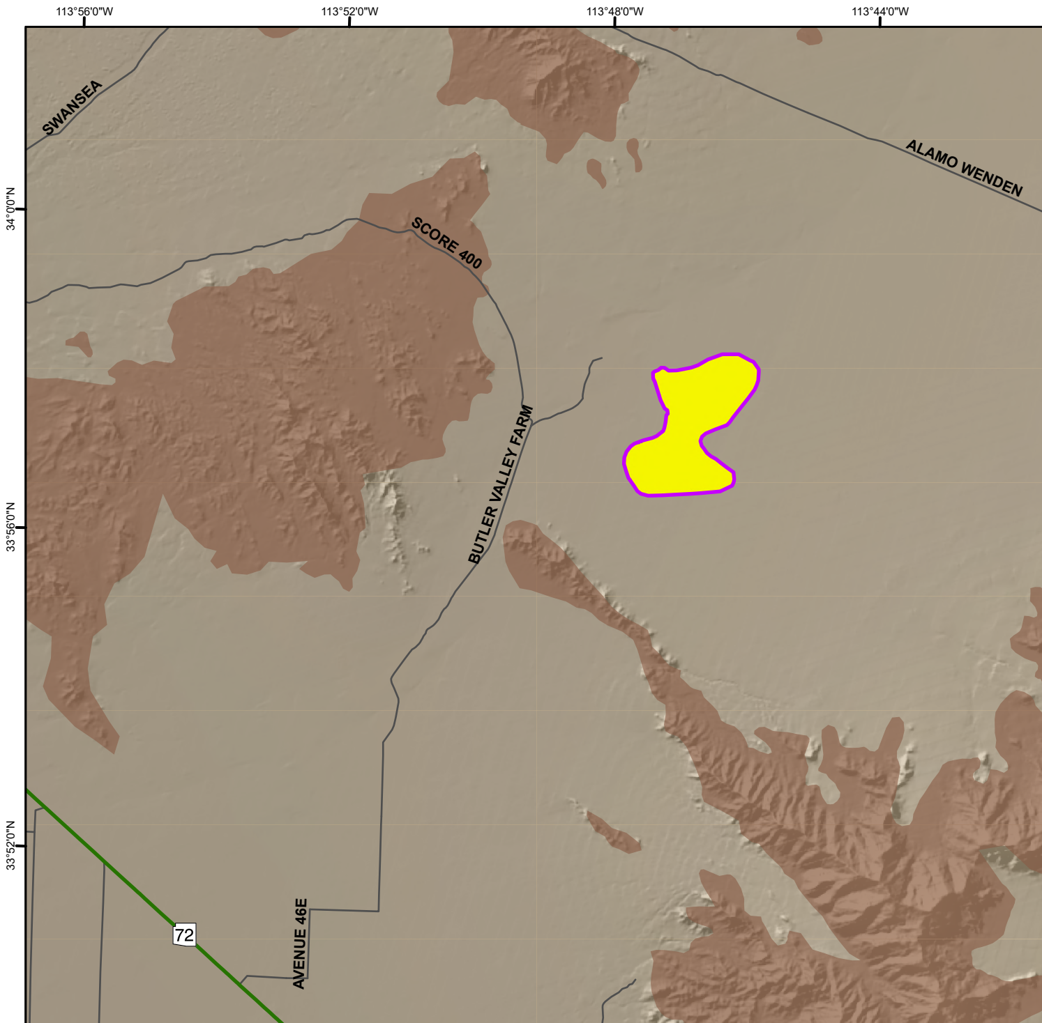
Total Land Subsidence in the Butler Valley Area, La Paz County Based on Radarsat-2 Satellite Interferometric Synthetic Aperture Radar (InSAR) Data Time Period of Analysis: 1.0 Years 03/31/2025 To 03/26/2026
