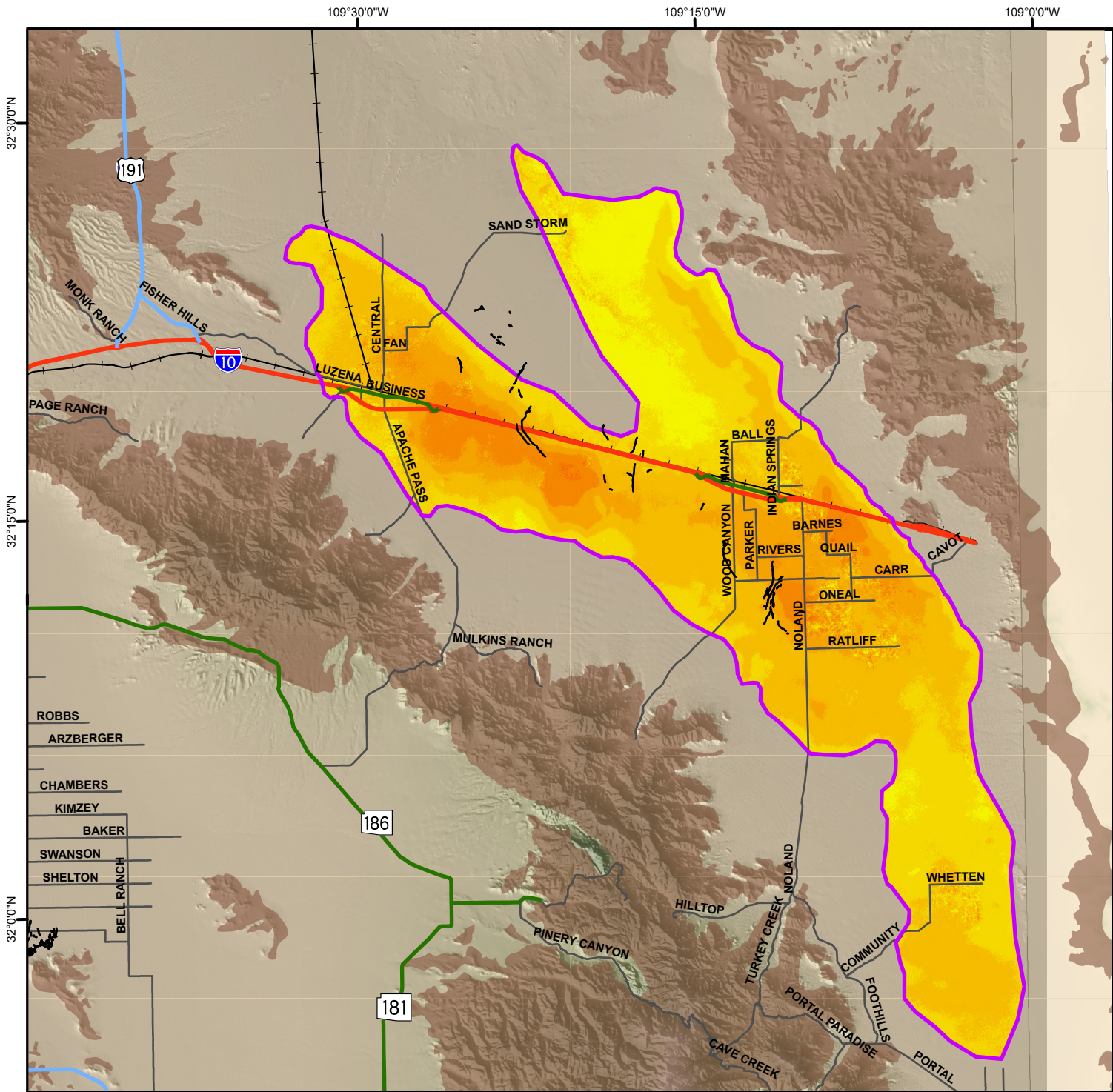
Total Land Subsidence in the Bowie and San Simon Areas, Cochise County Based on Sentinel-1 Satellite Interferometric Synthetic Aperture Radar (InSAR) Data Time Period of Analysis: 2.0 Years 05/13/2025 To 05/08/2026
