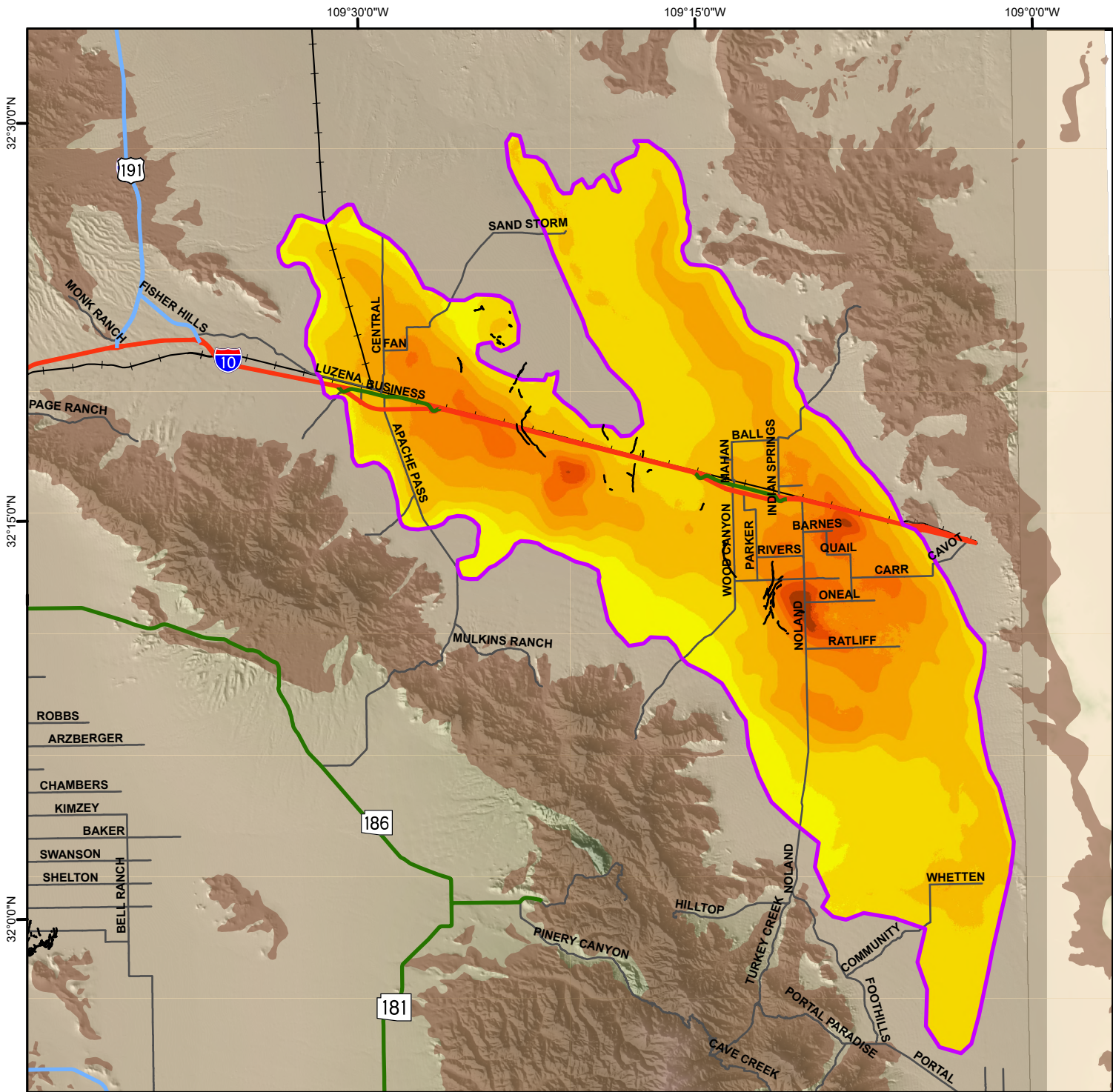
Total Land Subsidence in the Bowie and San Simon Areas, Cochise County Based on Radarsat-2 Satellite Interferometric Synthetic Aperture Radar (InSAR) Data Time Period of Analysis: 16.0 Years 05/05/2010 To 03/30/2026
