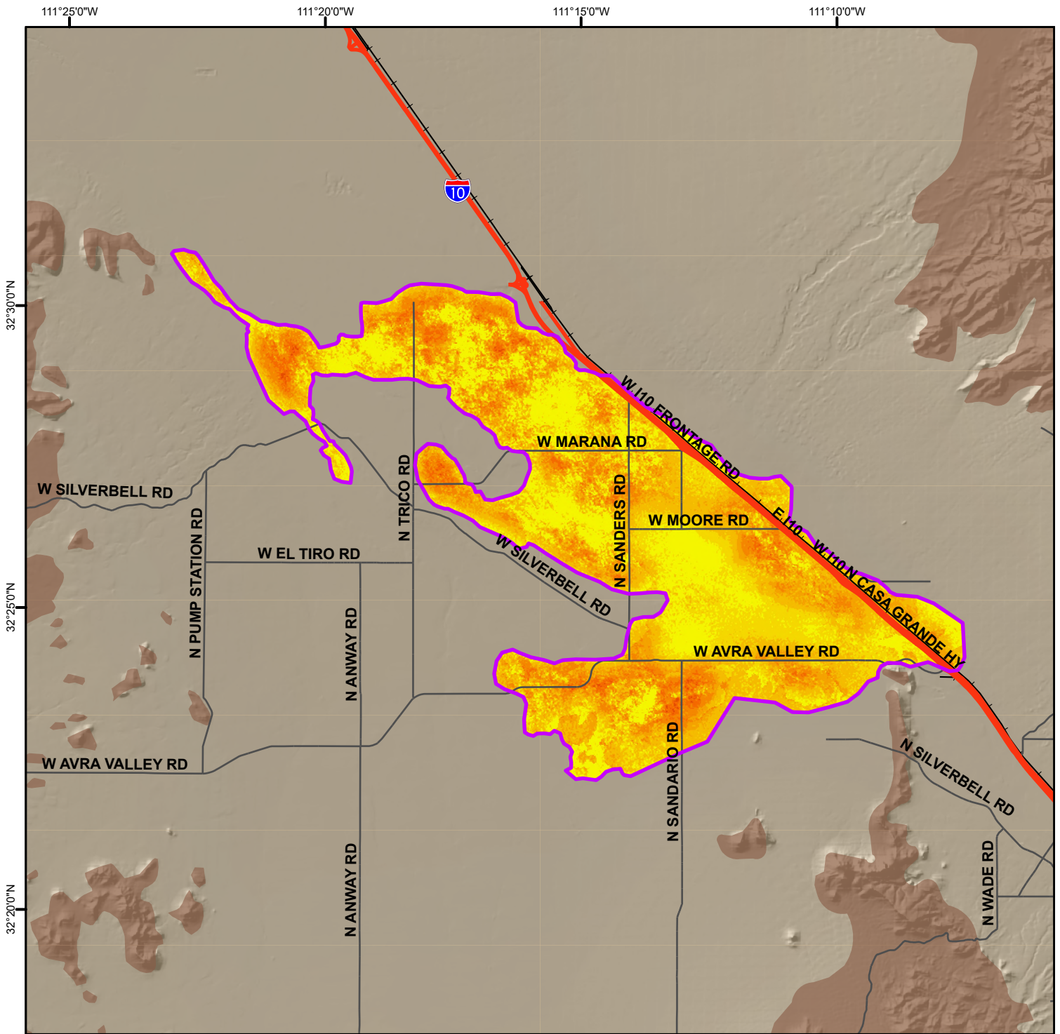
Total Land Subsidence in the Avra Valley Sub-basin Based on Radarsat-2 Satellite Interferometric Synthetic Aperture Radar (InSAR) Data Time Period of Analysis: 16.0 Years 05/15/2010 To 03/16/2026
