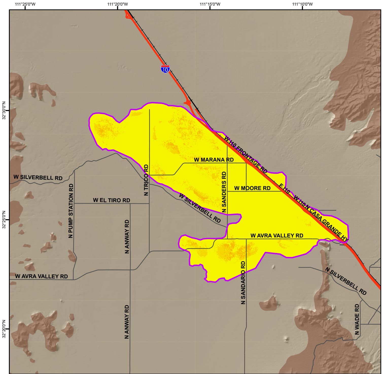
Total Land Subsidence in the Avra Valley Sub-basin Based on Radarsat-2 Satellite Interferometric Synthetic Aperture Radar (InSAR) Data Time Period of Analysis: 1.0 Years 03/21/2025 To 03/16/2026
