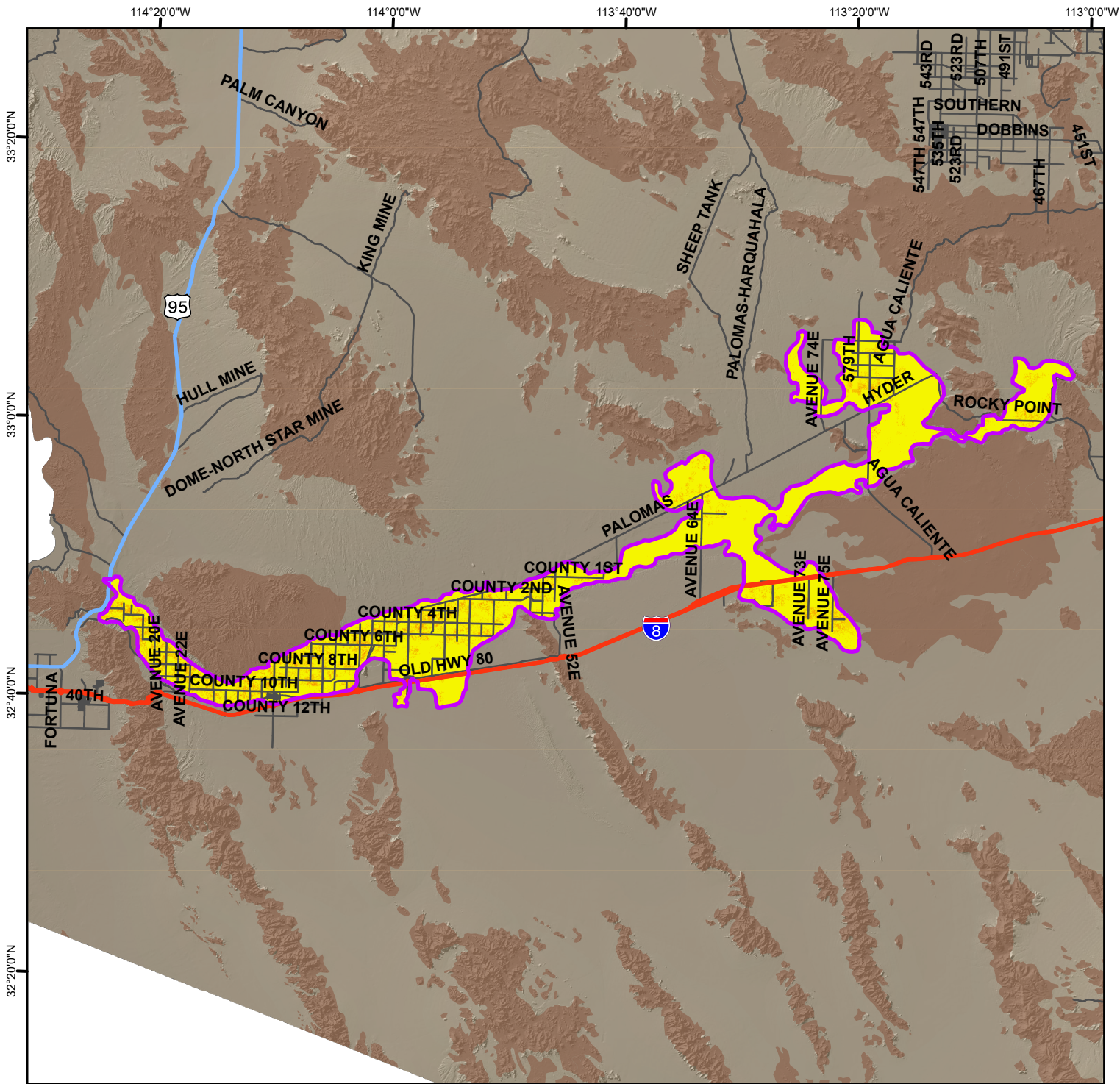
Total Land Subsidence in the Lower Gila Area, Maricopa and Yuma Counties Based on Sentinel-1 Satellite Interferometric Synthetic Aperture Radar (InSAR) Data Time Period of Analysis: 1.0 Years 05/04/2024 To 05/23/2025
