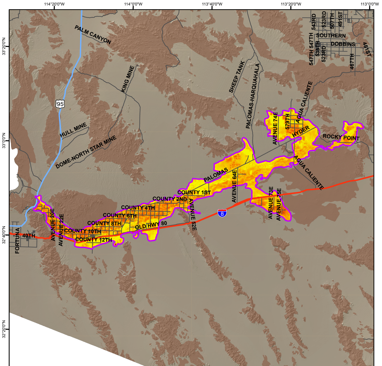
Total Land Subsidence in the Lower Gila Area, Maricopa and Yuma Counties Based on Sentinel-1 Satellite Interferometric Synthetic Aperture Radar (InSAR) Data Time Period of Analysis: 8.0 Years 04/23/2017 To 05/23/2025
