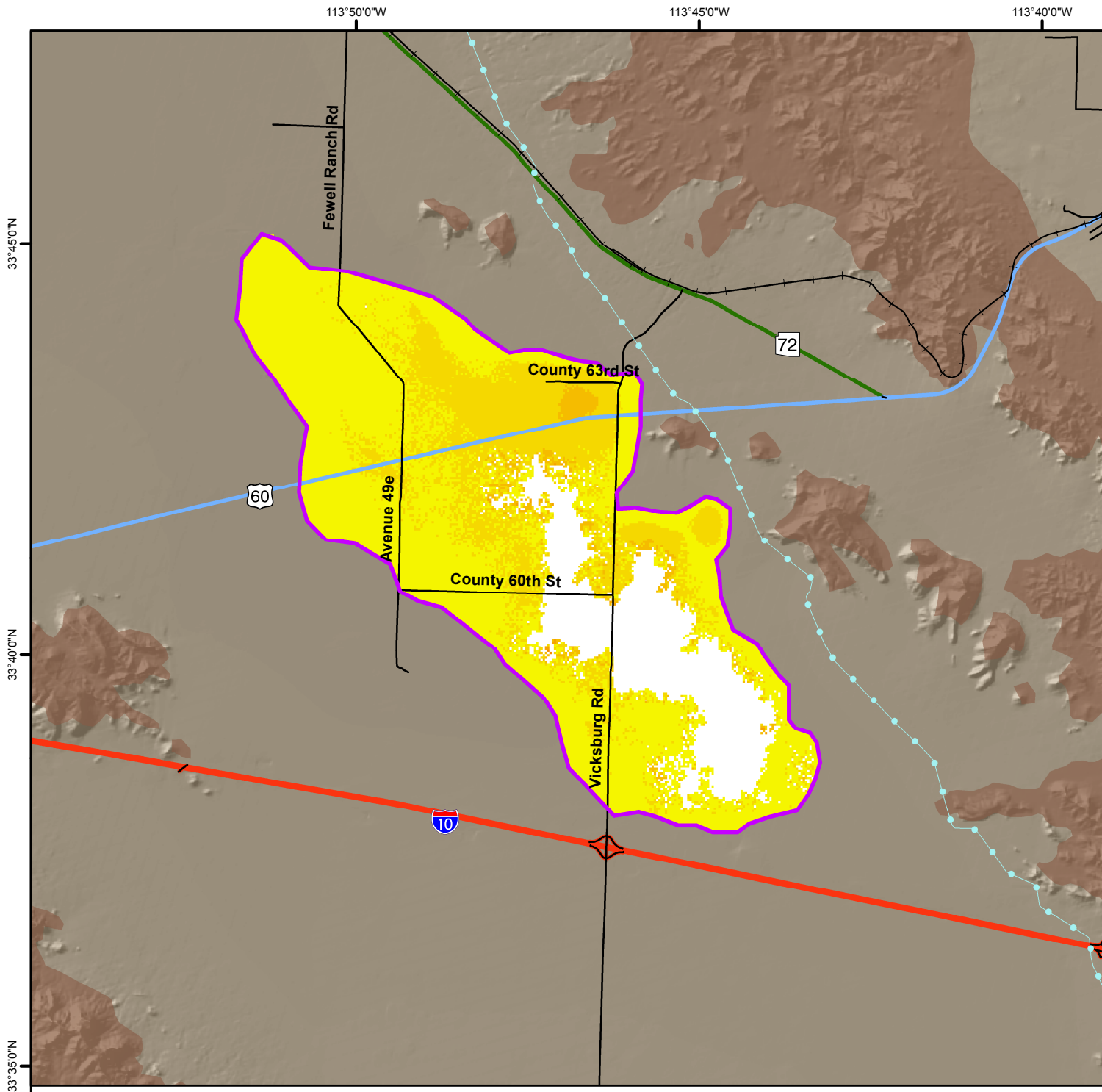
Total Land Subsidence in the Ranegras Valley, La Paz County Based on Radarsat-2 Satellite Interferometric Synthetic Aperture Radar (InSAR) Data Time Period of Analysis: 1.9 Years 05/01/2010 To 03/27/2012
