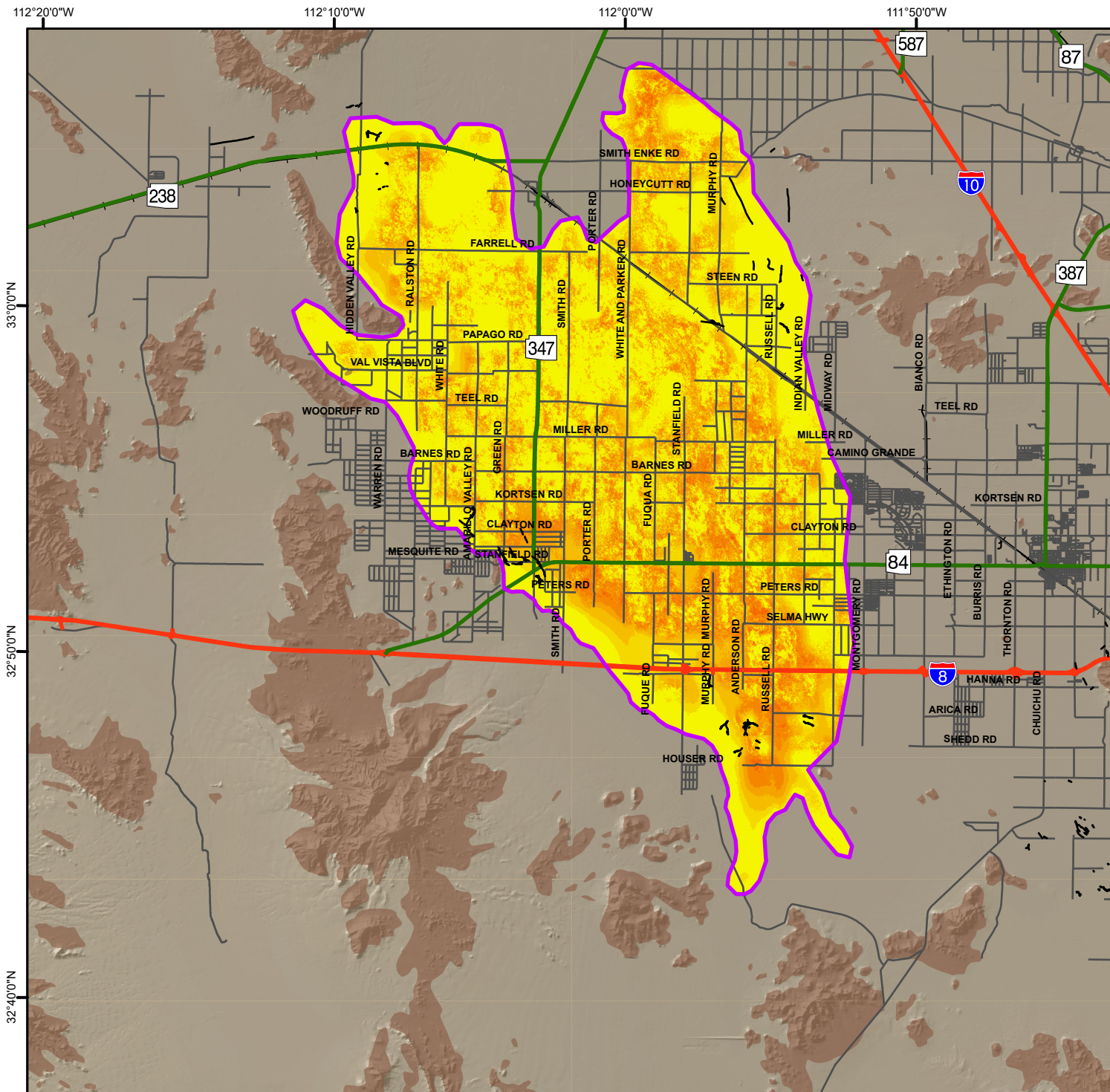
Total Land Subsidence in the Maricopa-Stanfield Sub-Basin, Pinal County Based on Radarsat-2 Satellite Interferometric Synthetic Aperture Radar (InSAR) Data Time Period of Analysis: 11.9 Years 05/08/2010 To 03/30/2022
