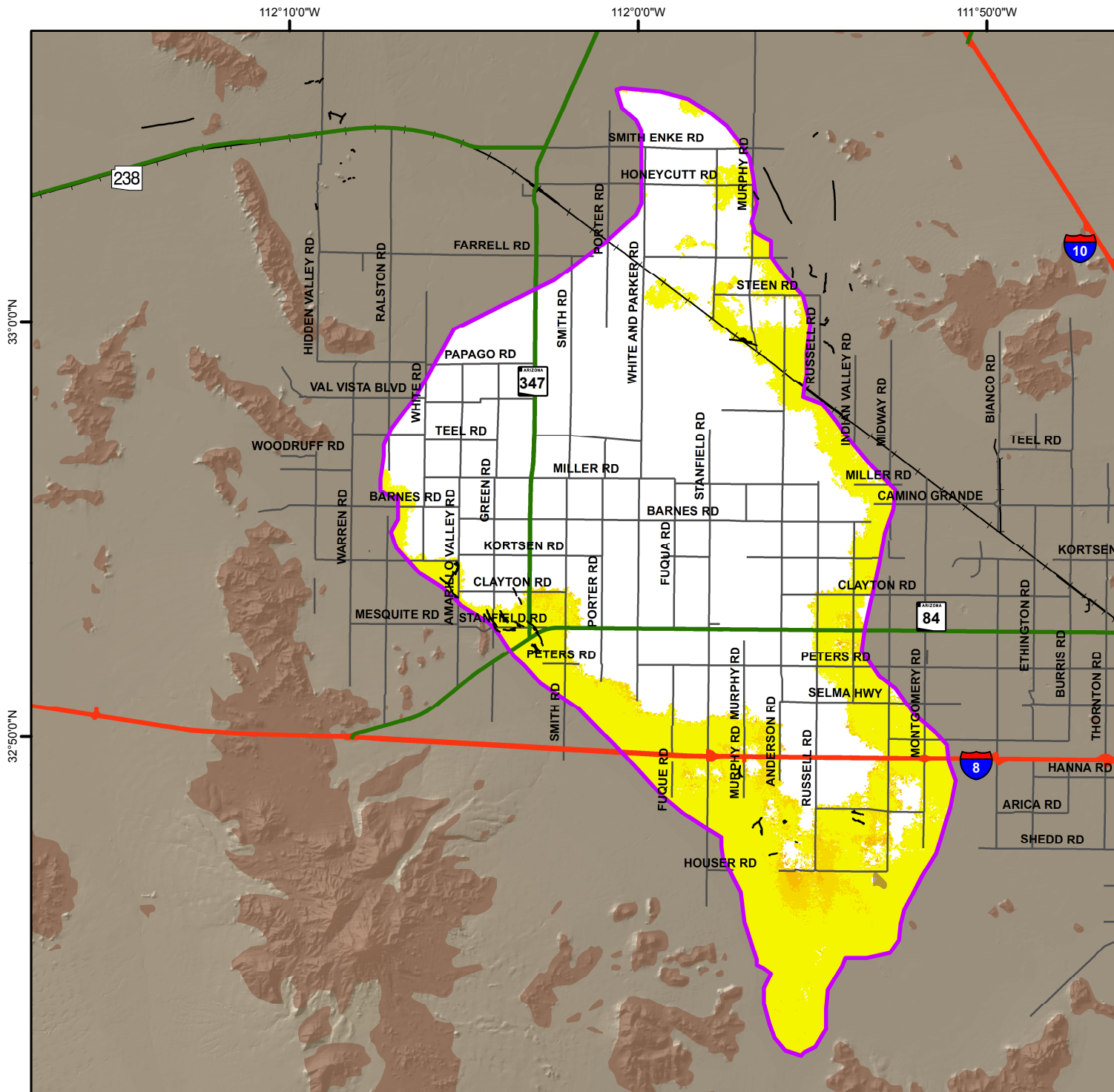
Total Land Subsidence in the Maricopa-Stanfield Sub-Basin, Pinal County Based on Envisat Satellite Interferometric Synthetic Aperture Radar (InSAR) Data Time Period of Analysis: 1.9 Years 04/18/2007 To 02/27/2008
