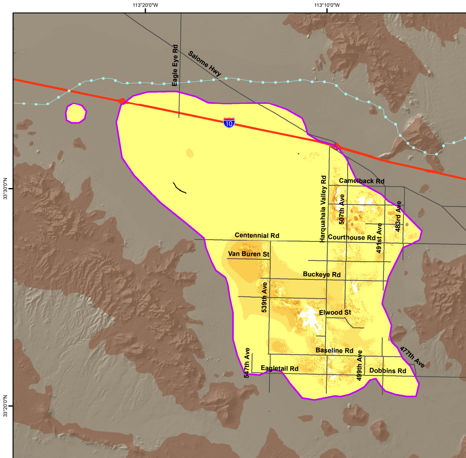
Land Subsidence Rate in the Harquahala Valley, Maricopa County Based on Radarsat-2 Satellite Interferometric Synthetic Aperture Radar (InSAR) Data Time Period of Analysis: 1.0 Years 04/08/2019 To 04/26/2020
