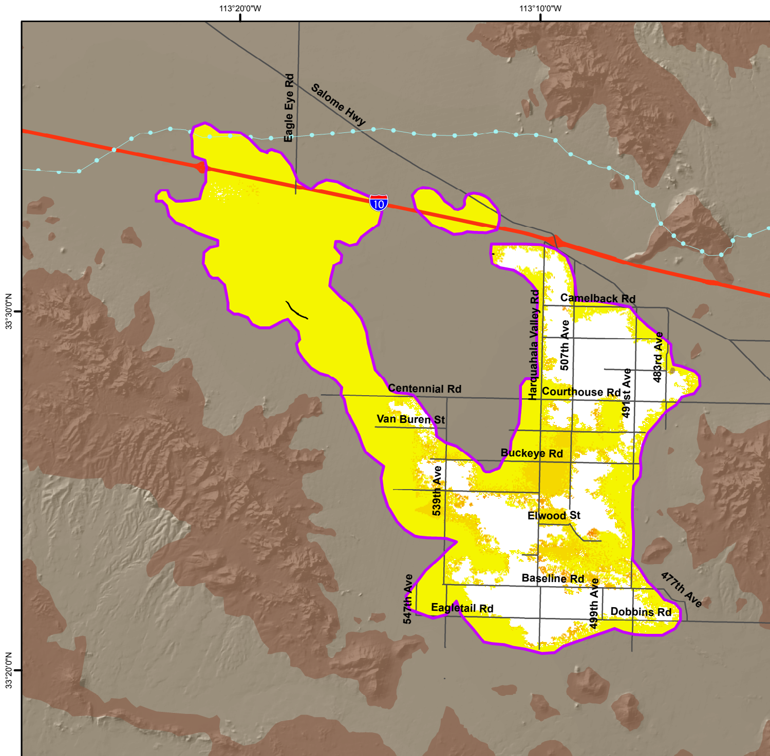
Total Land Subsidence in the Harquahala Valley, Maricopa County Based on Envisat Satellite Interferometric Synthetic Aperture Radar (InSAR) Data Time Period of Analysis: 2.0 Years 02/14/2007 To 02/18/2009
